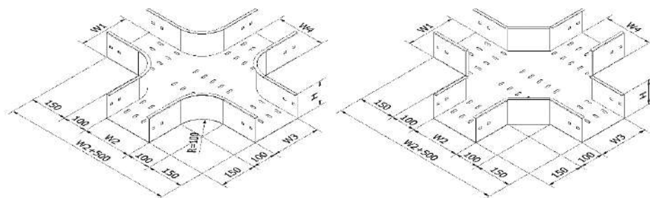
Cross elbow W \geq 200
