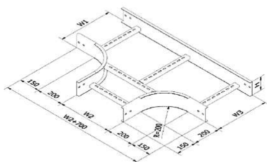
Tee elbow W≥400
