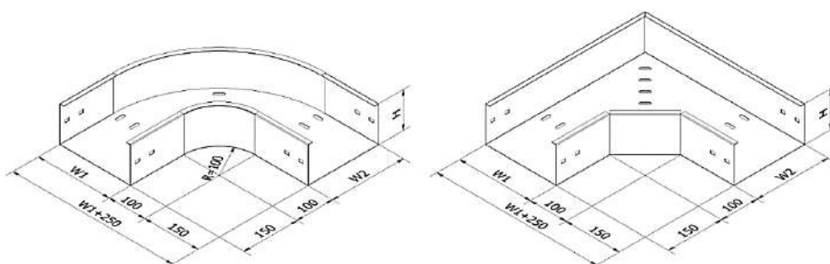
Horizontal elbow W \geq 200
