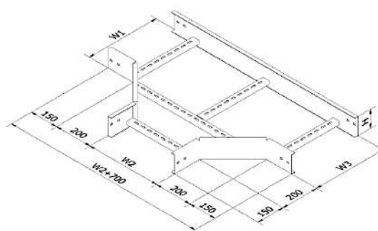
Tee elbow W≥400
