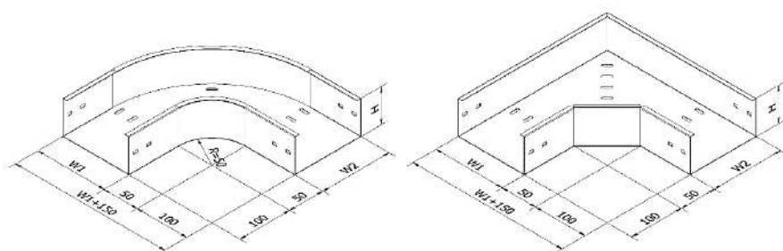
Horizontal elbow W < 200
