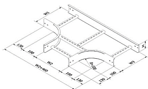
Tee elbow W<400
