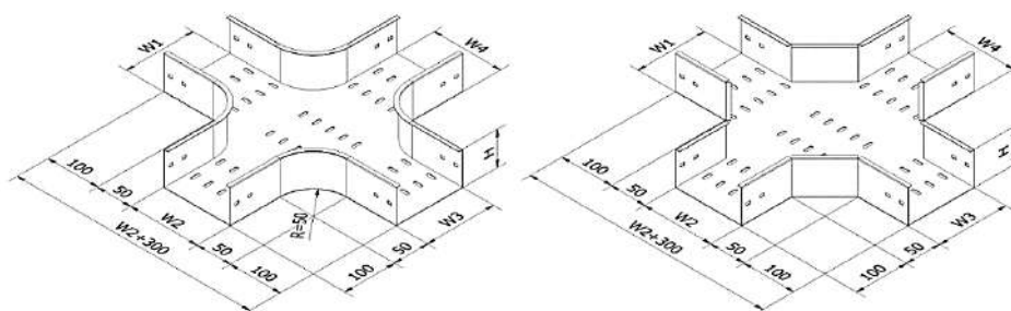
Cross elbow W < 200
