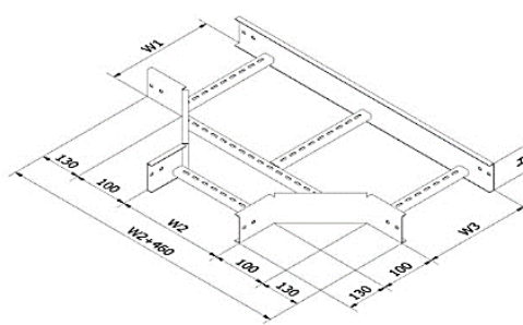
Tee elbow W<400
